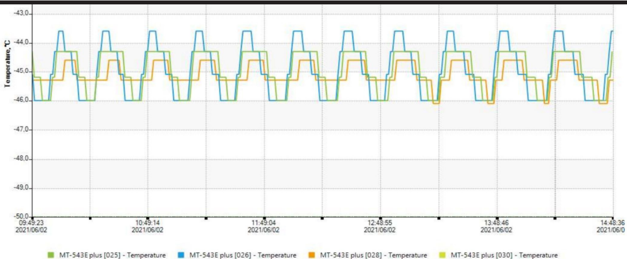
PERFORMANCE DATA GRAPH: This Graph Illustrates The MED430CLF's Temperature Range Down To -45°C .
