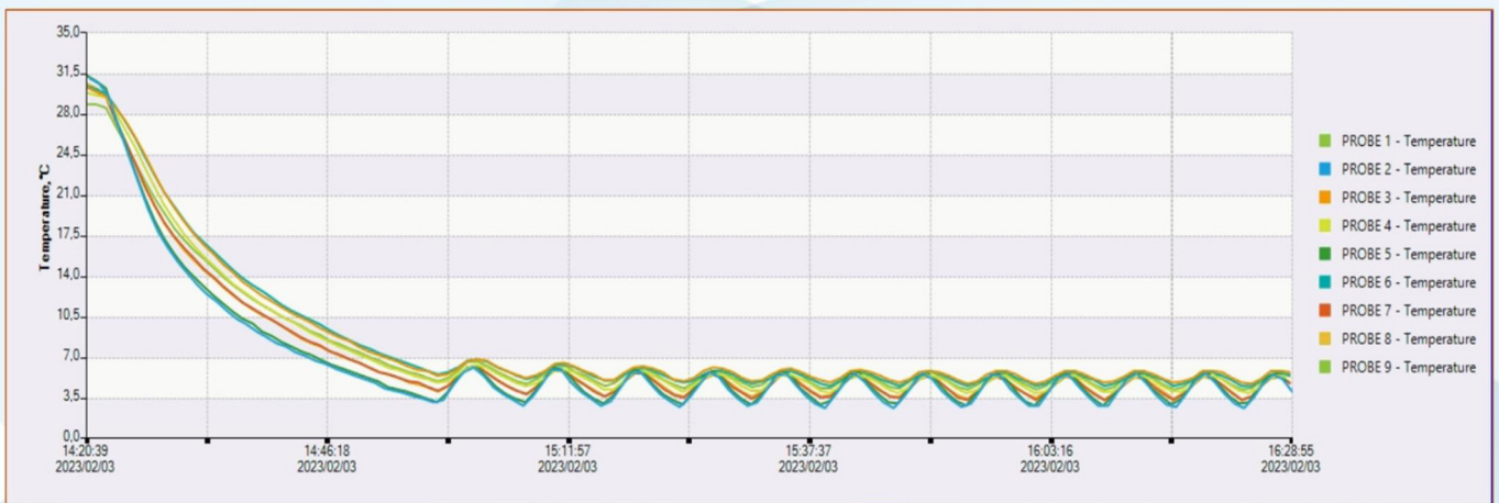
PERFORMANCE DATA GRAPH: How The MED400GHD Maintains Temperature Between 2°C And 8°C At 32°C Ambient Temperature
