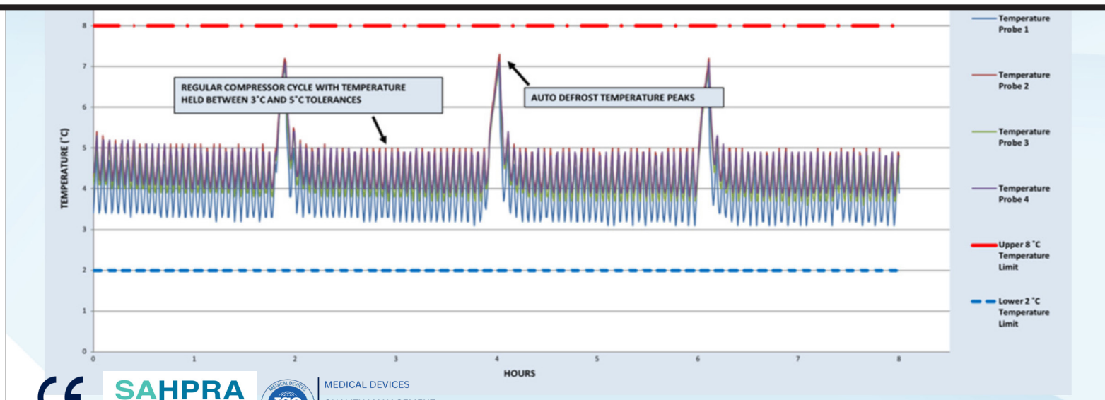
PERFORMANCE DATA GRAPH: How The MED250GHD Maintains Temperature Between 3°C And 5°C At 32°C Ambient Temperature
