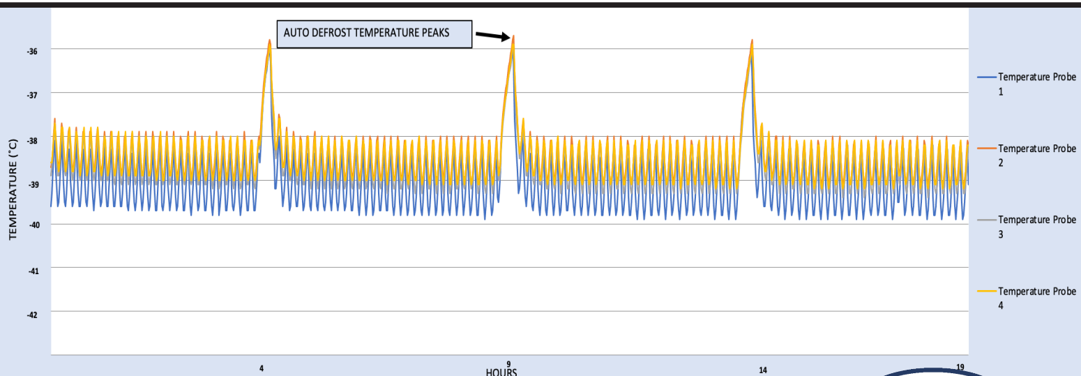
PERFORMANCE DATA GRAPH: LAB470SLF Temperature Performance At 32°C Ambient Temperature
