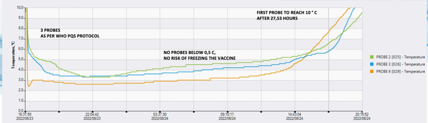
PERFORMANCE DATA GRAPH: This Graph Indicates The Excellent Temperature Performance Of The Vaccine Carrier VB03 At 43°C
