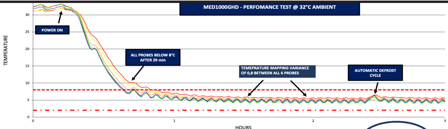
PERFORMANCE DATA GRAPH: How The MED1000GHD Maintains Temperature Between 2°C And 8°C At 32°C Ambient Temperature
